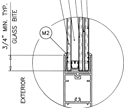
GLASS TYPE 'A1' 1" OVERALL INSUL. LAM. GLASS
