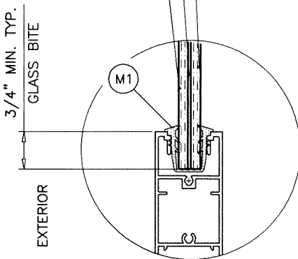
GLASS TYPE 'A' 7/16" OVERALL LAM. GLASS
